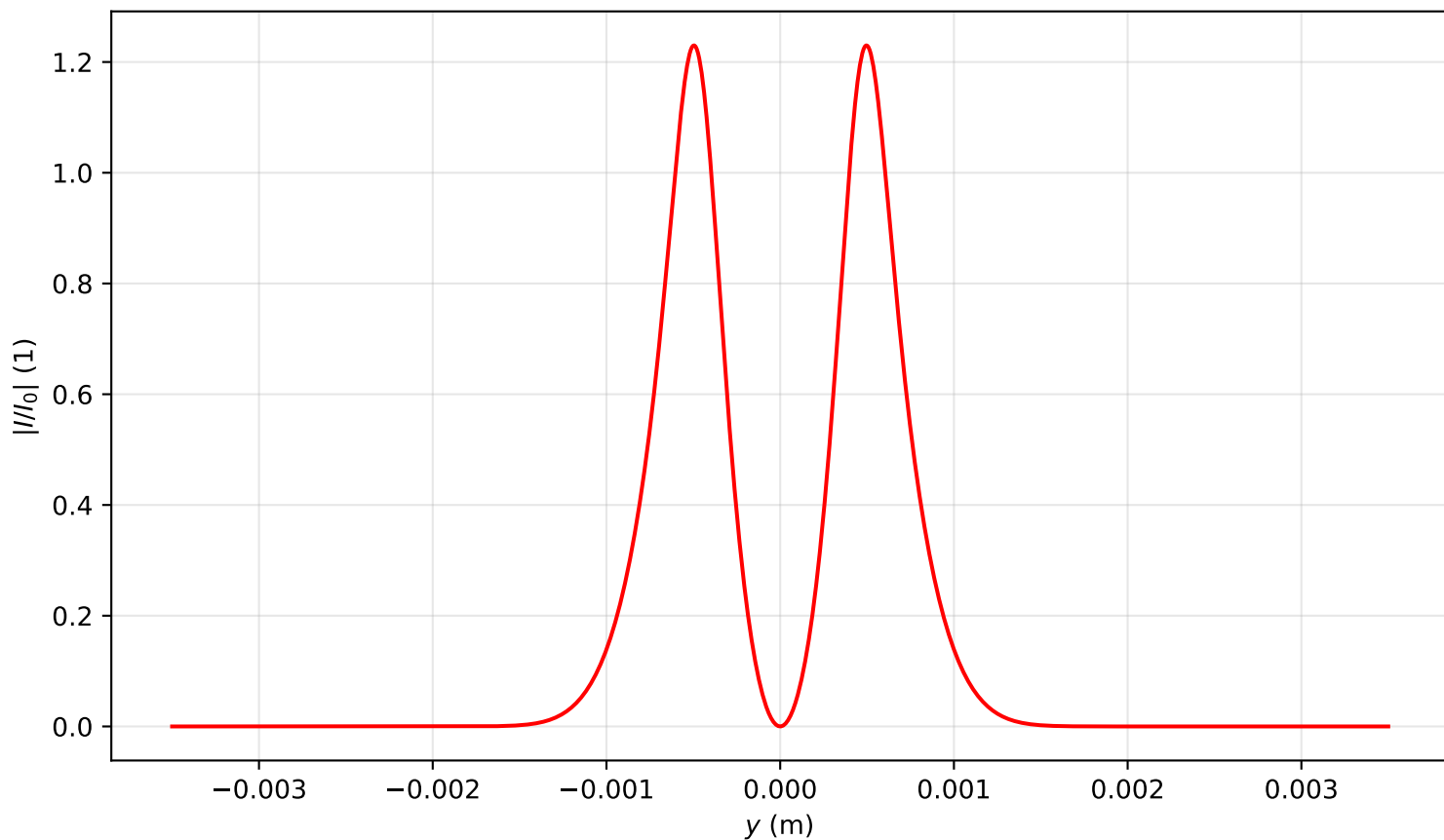
Intensity profile I(x=0, y, z=0.239)/I_0 , P_{in}=9.0P_{cr} , artificial time
